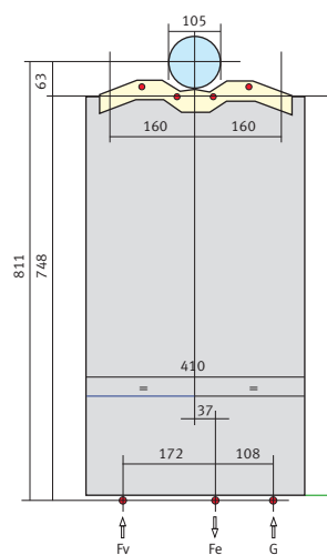
ThemaClassic AS
